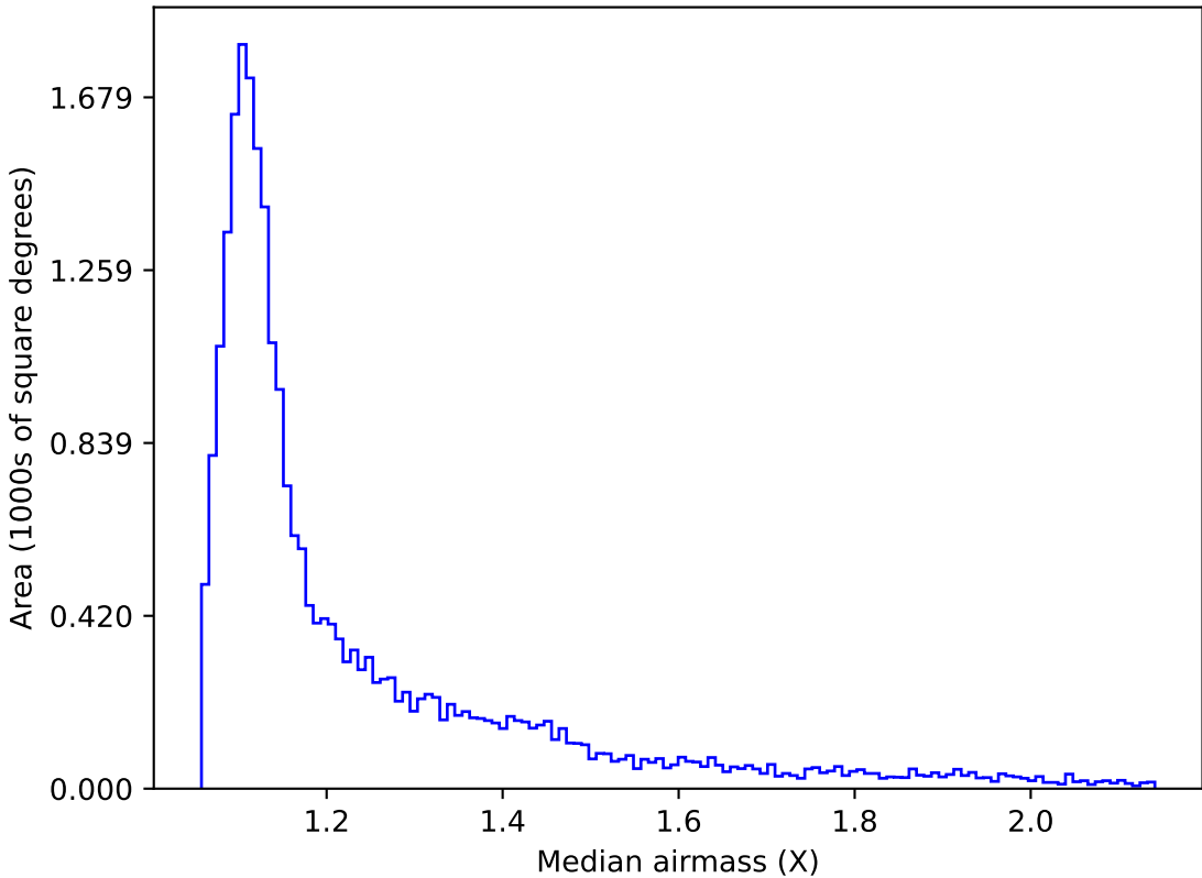
ddf_acor_sf15_lsf20_lsr50_v3.4_10yrs Yr 1 i band: Median airmass
