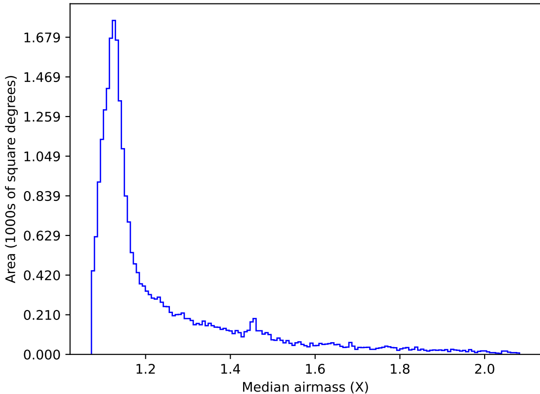
ddf_acor_sf15_lsf20_lsr50_v3.4_10yrs Yr 1 all bands: Median airmass
