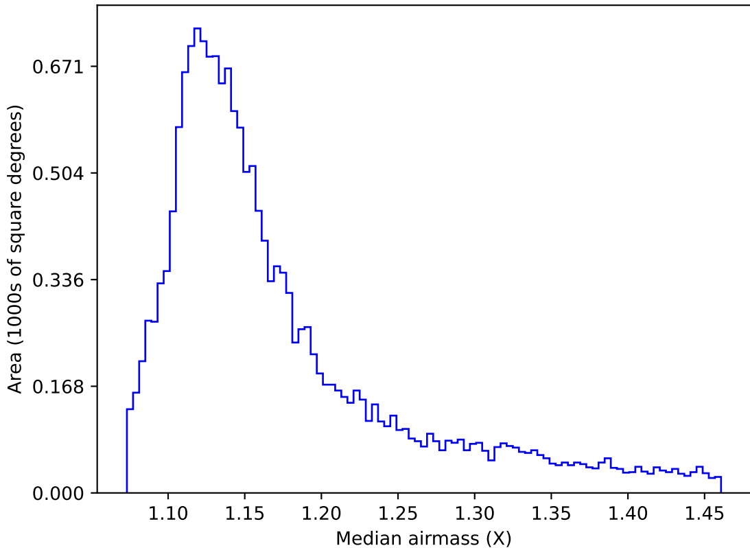
ddf_acor_sf15_lsf20_lsr50_v3.4_10yrs WFD u band: Median airmass
