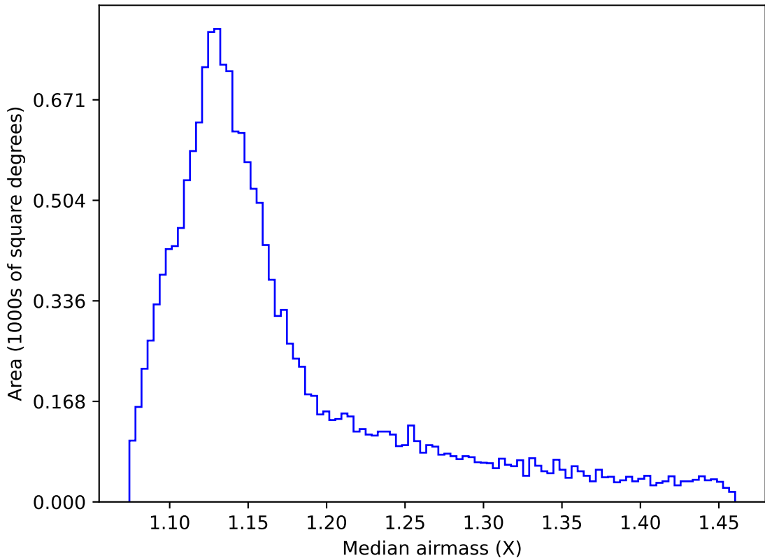
ddf_acor_sf15_lsf20_lsr50_v3.4_10yrs WFD r band: Median airmass
