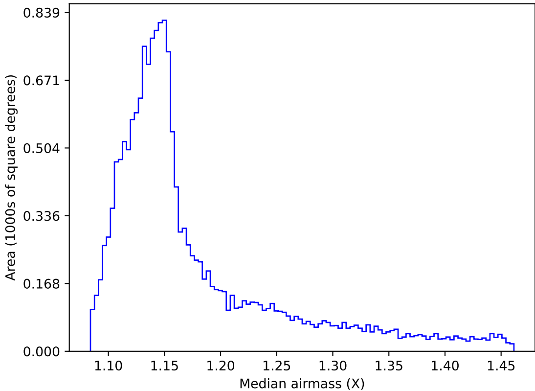
ddf_acor_sf15_lsf20_lsr50_v3.4_10yrs WFD all bands: Median airmass
