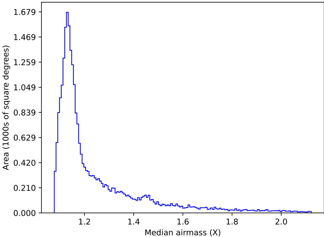
ddf_acor_sf15_lsf20_lsr50_v3.4_10yrs All sky r band: Median airmass
