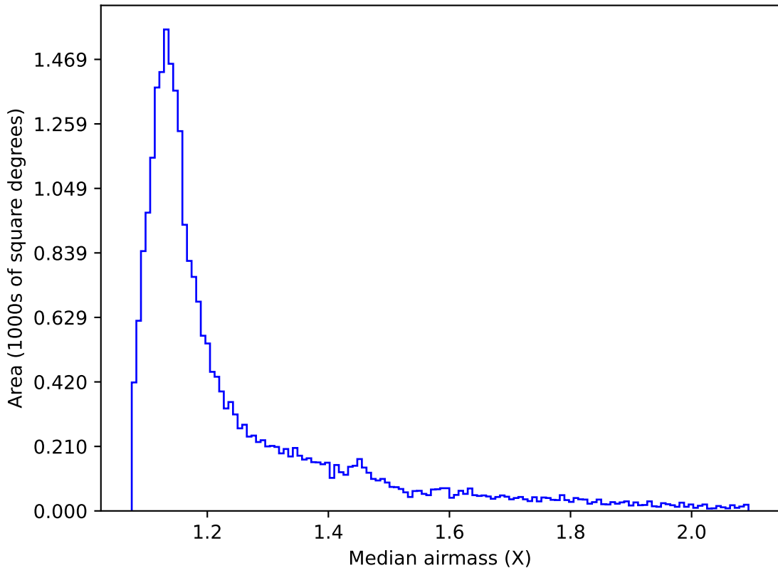
ddf_acor_sf15_lsf20_lsr50_v3.4_10yrs All sky g band: Median airmass
