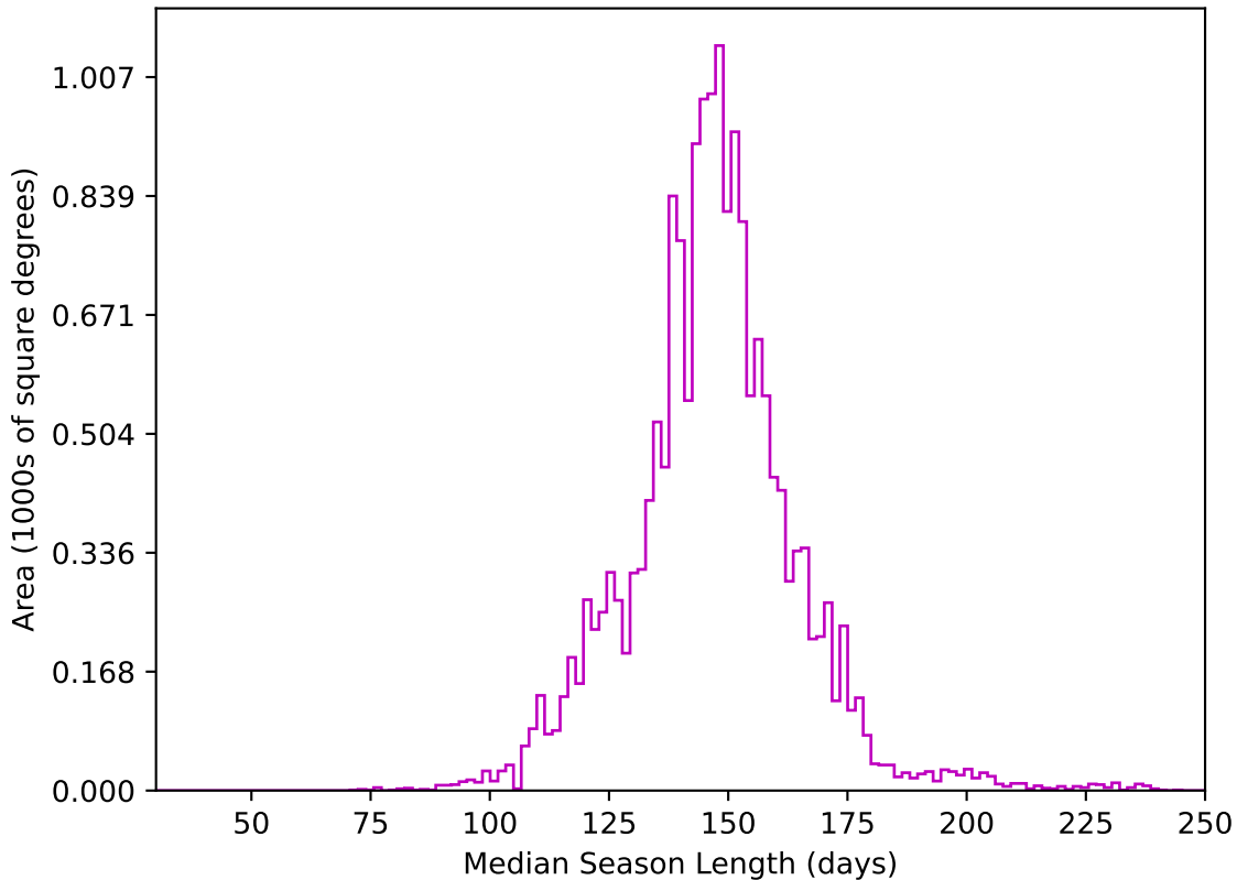
ddf_acor_sf15_lsf20_lsr50_v3.4_10yrs WFD z band: Median Season Length
