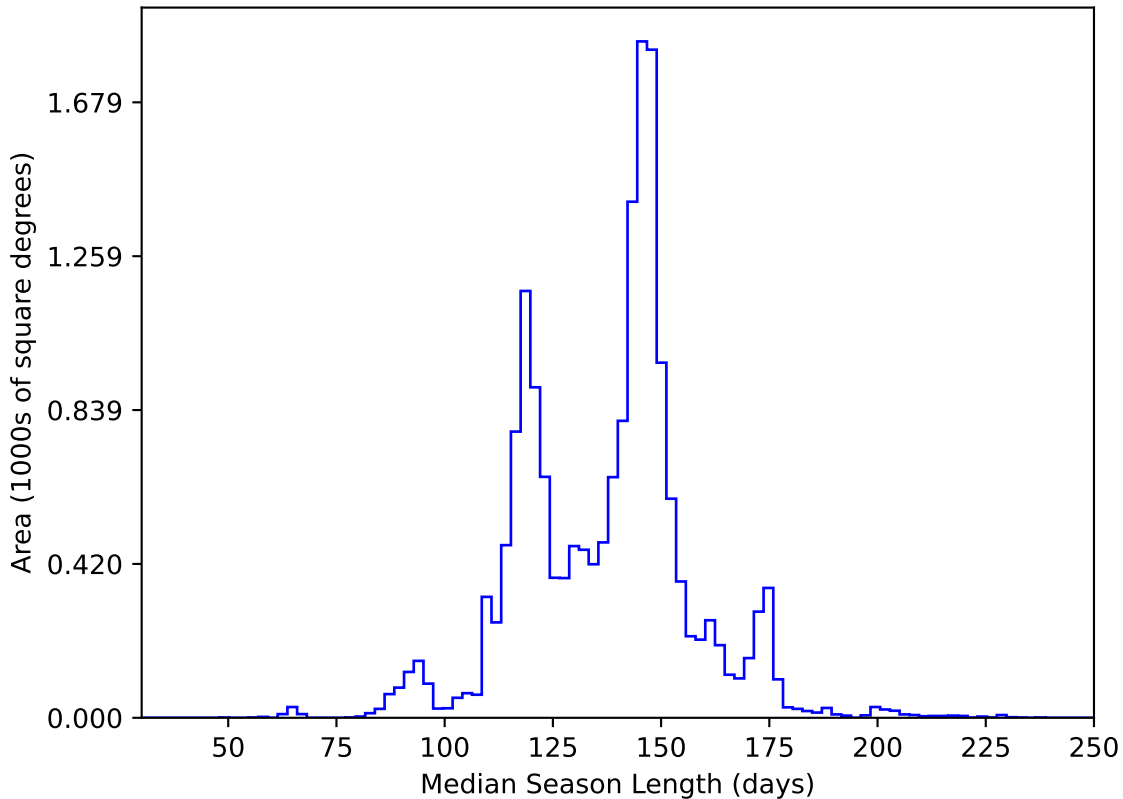
ddf_acor_sf15_lsf20_lsr50_v3.4_10yrs WFD y band: Median Season Length
