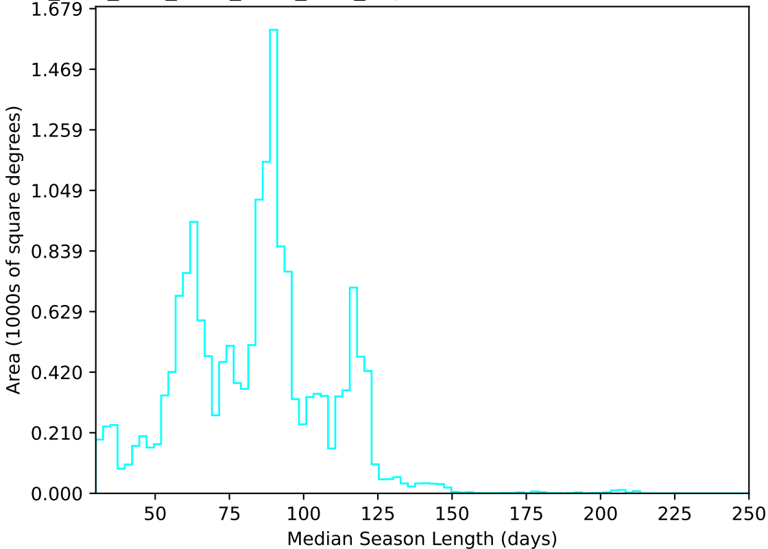
ddf_acor_sf15_ls20_lsr50_v3.4_10yrs WFD u band: Median Season Length
