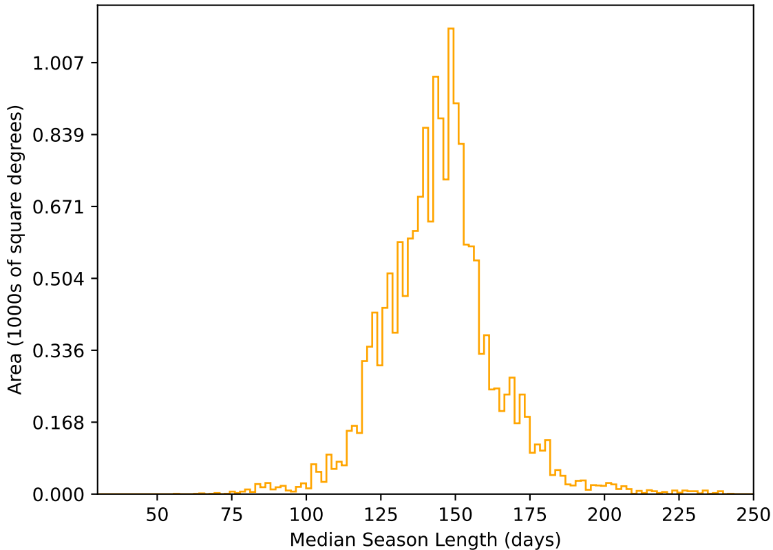
ddf_acor_sf15_lsf20_lsr50_v3.4_10yrs WFD r band: Median Season Length
