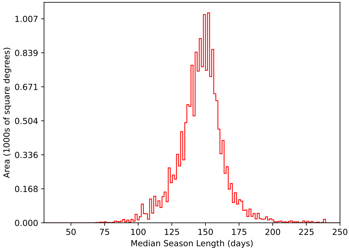
ddf_acor_sf15_lsf20_lsr50_v3.4_10yrs WFD i band: Median Season Length
