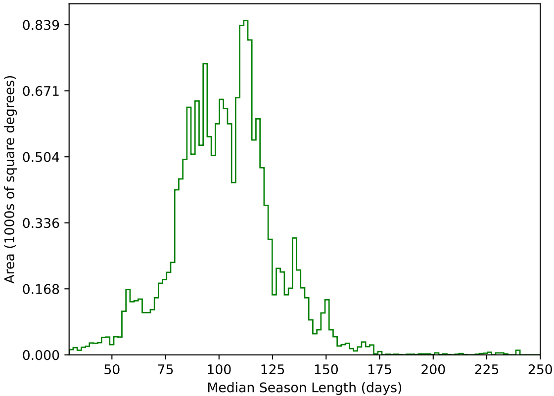
ddf_acor_sf15_lsf20_lsr50_v3.4_10yrs WFD g band: Median Season Length
