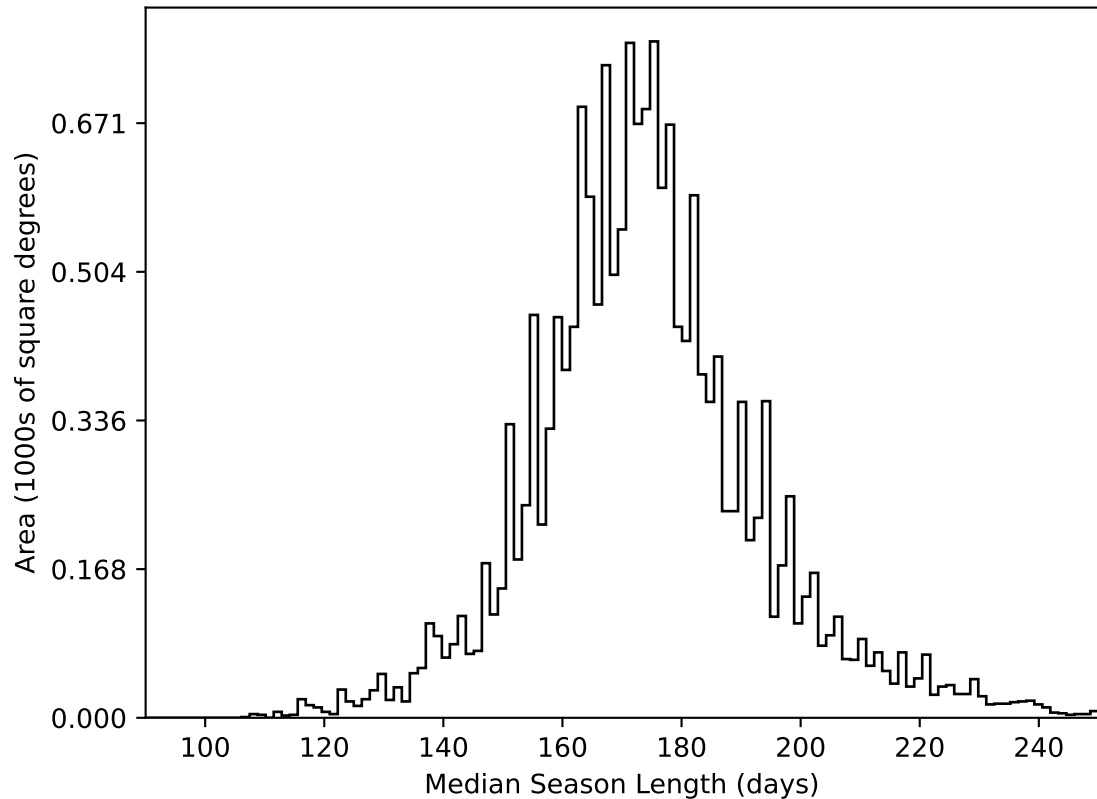
ddf_acor_sf15_lsf20_lsr50_v3.4_10yrs WFD all bands: Median Season Length
