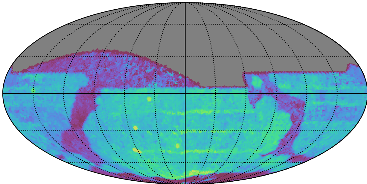
ddf_acor_sf15_lsf20_lsr50_v3.4_10yrs All sky z band: Median Season Length
