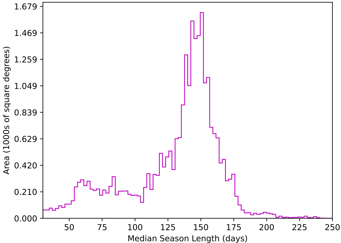
ddf_acor_sf15_lsf20_lsr50_v3.4_10yrs All sky z band: Median Season Length
