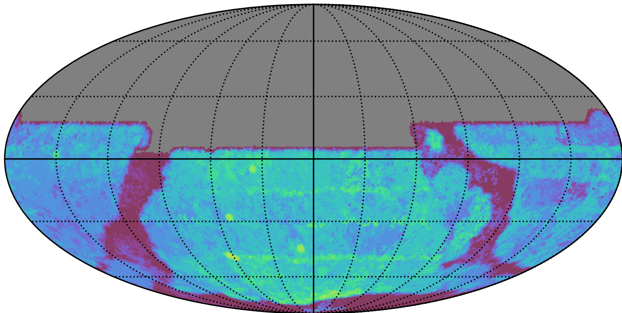
ddf_acor_sf15_lsf20_lsr50_v3.4_10yrs All sky y band: Median Season Length
