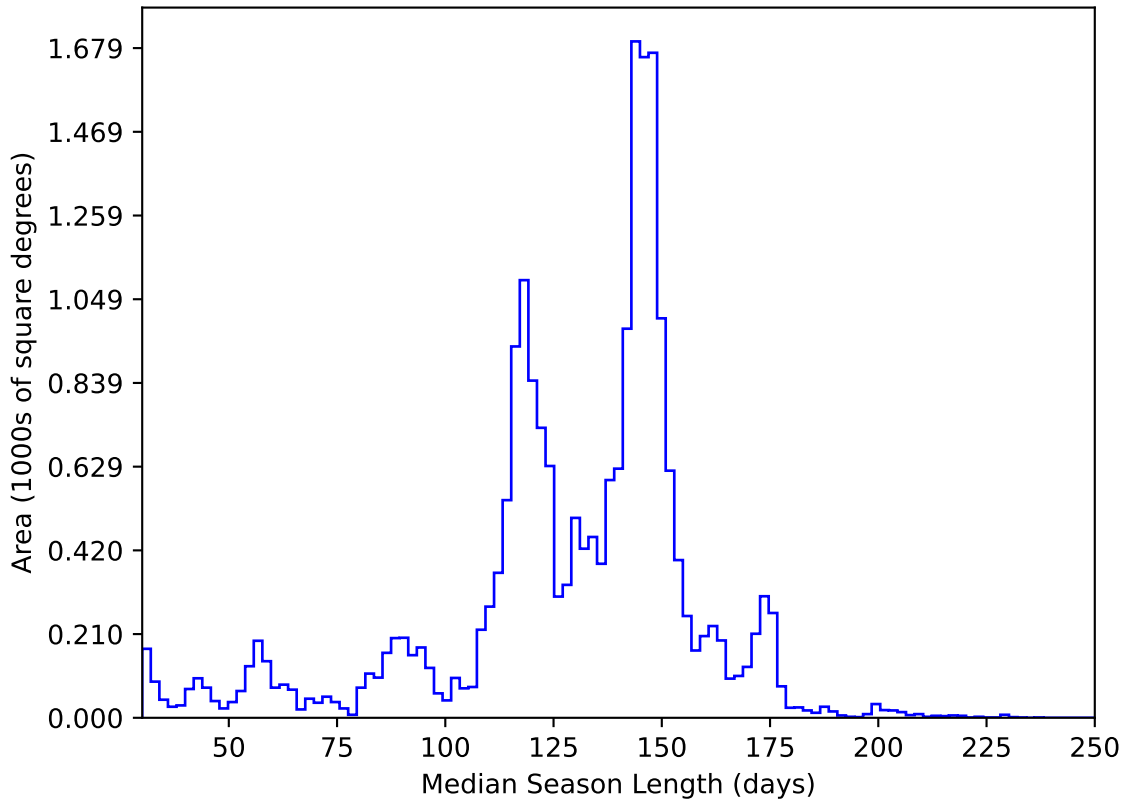
ddf_acor_sf15_lsf20_lsr50_v3.4_10yrs All sky y band: Median Season Length
