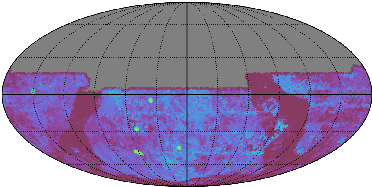
ddf_acor_sf15_lsf20_lsr50_v3.4_10yrs All sky u band: Median Season Length
