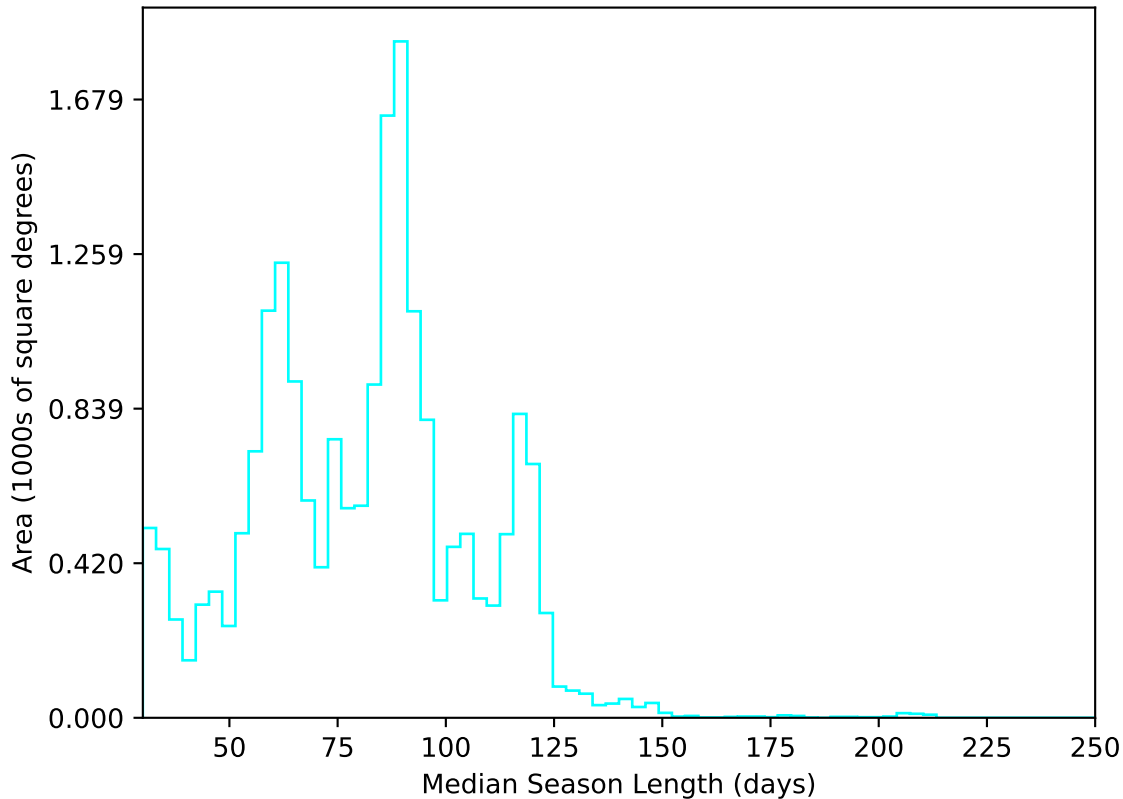
ddf_acor_sf15_lsf20_lsr50_v3.4_10yrs All sky u band: Median Season Length
