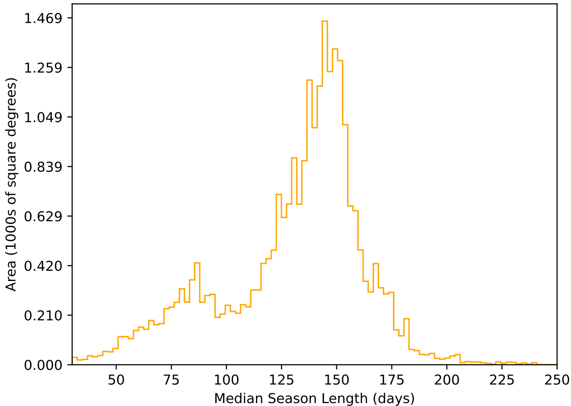
ddf_acor_sf15_lsf20_lsr50_v3.4_10yrs All sky r band: Median Season Length
