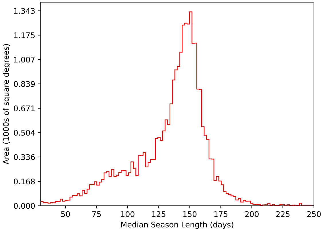
ddf_acor_sf15_lsf20_lsr50_v3.4_10yrs All sky i band: Median Season Length
