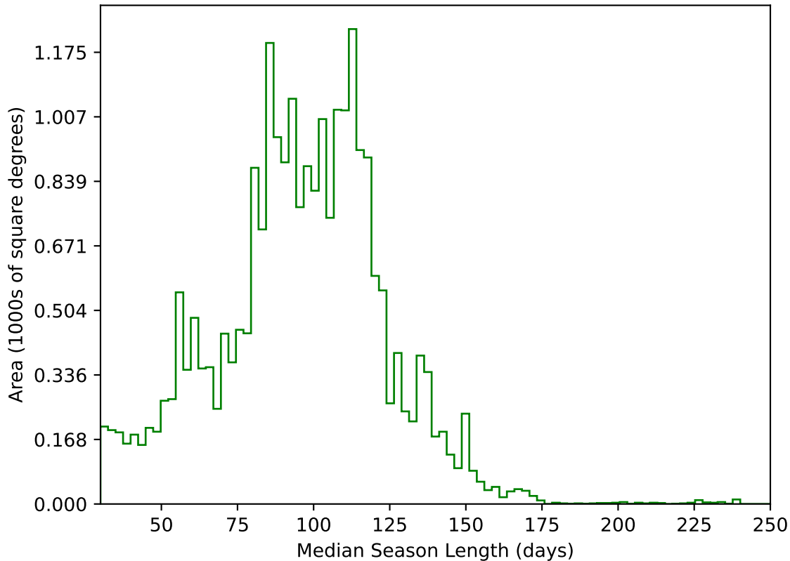
ddf_acor_sf15_lsf20_lsr50_v3.4_10yrs All sky g band: Median Season Length
