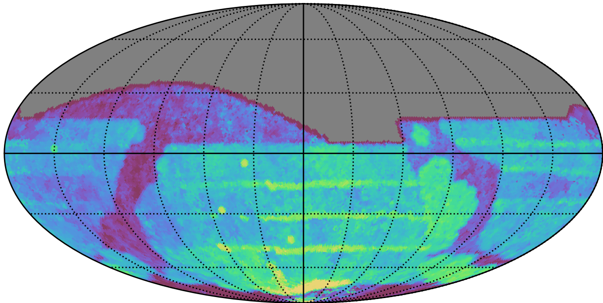
ddf_acor_sf15_lsf20_lsr50_v3.4_10yrs All sky all bands: Median Season Length
