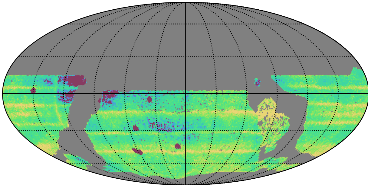
ddf_acor_sf15_lsf20_lsr50_v3.4_10yrs WFD: Median Intra-Night Gap
