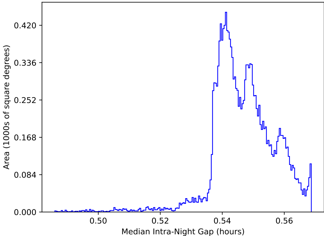
ddf_acor_sf15_lsf20_lsr50_v3.4_10yrs WFD: Median Intra-Night Gap
