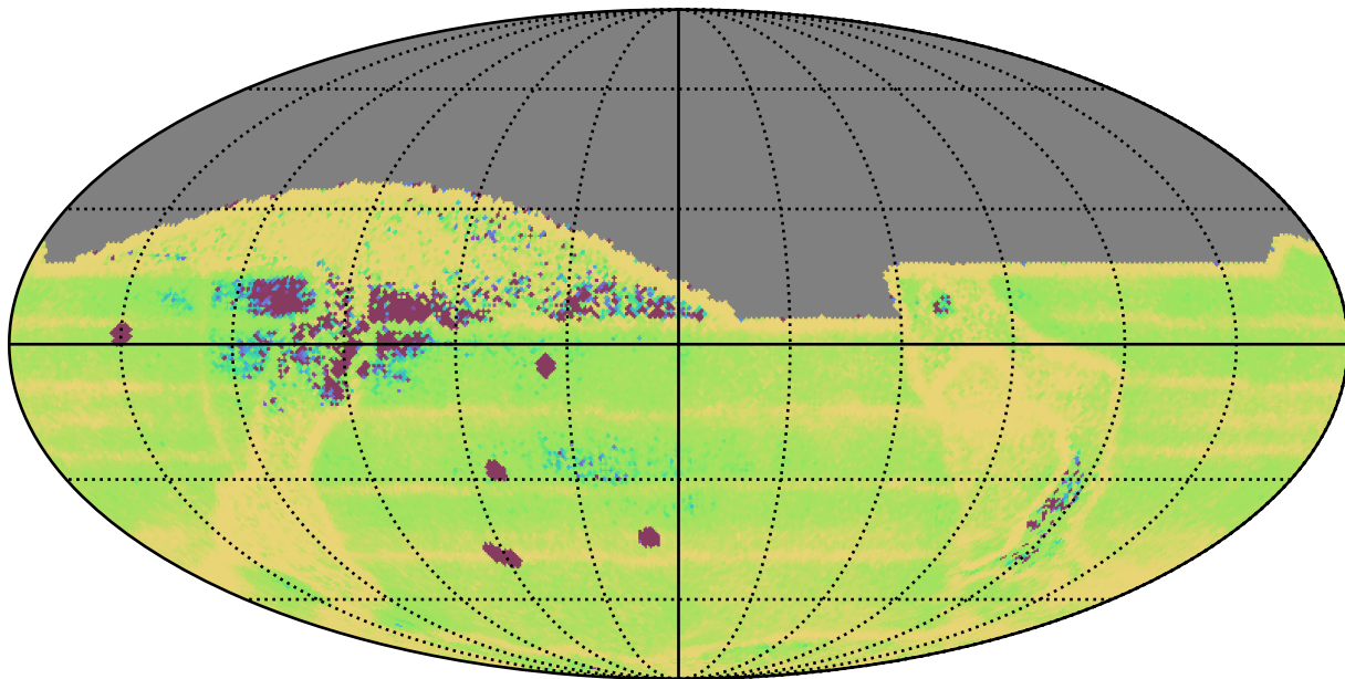
ddf_acor_sf15_lsf20_lsr50_v3.4_10yrs All sky: Median Intra-Night Gap
