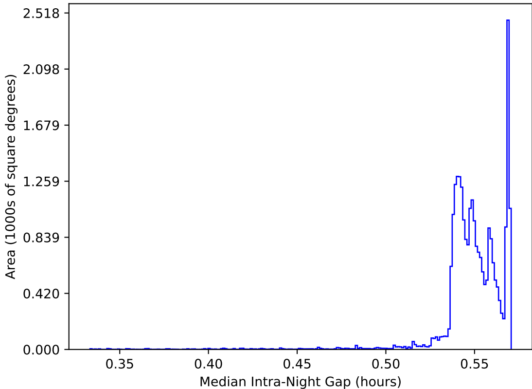
ddf_acor_sf15_lsf20_lsr50_v3.4_10yrs All sky: Median Intra-Night Gap
