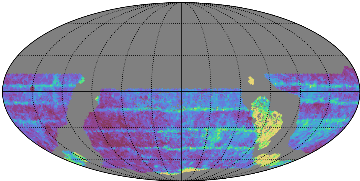
ddf_acor_sf15_lsf20_lsr50_v3.4_10yrs WFD z band: Median Inter-Night Gap
