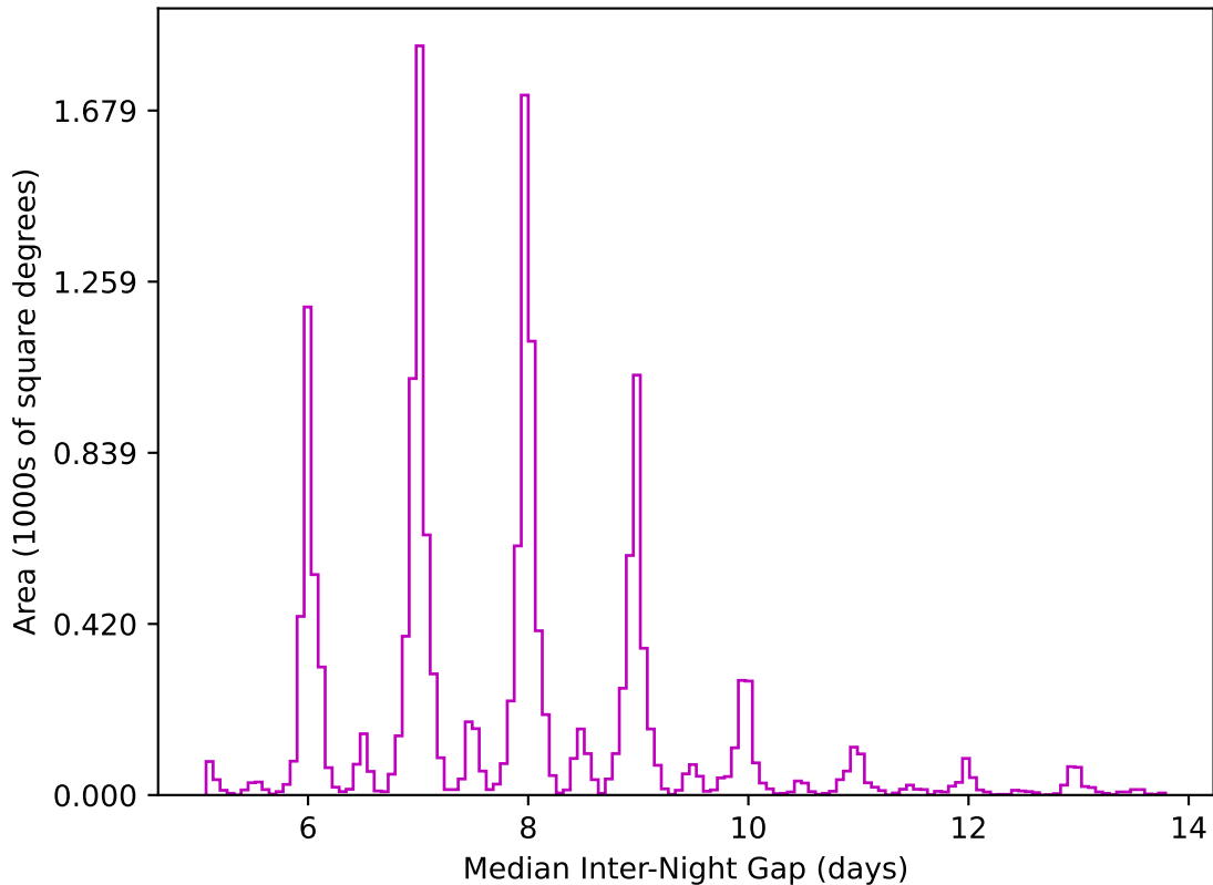
ddf_acor_sf15_lsf20_lsr50_v3.4_10yrs WFD z band: Median Inter-Night Gap
