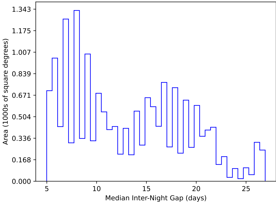
ddf_acor_sf15_lsf20_lsr50_v3.4_10yrs WFD y band: Median Inter-Night Gap
