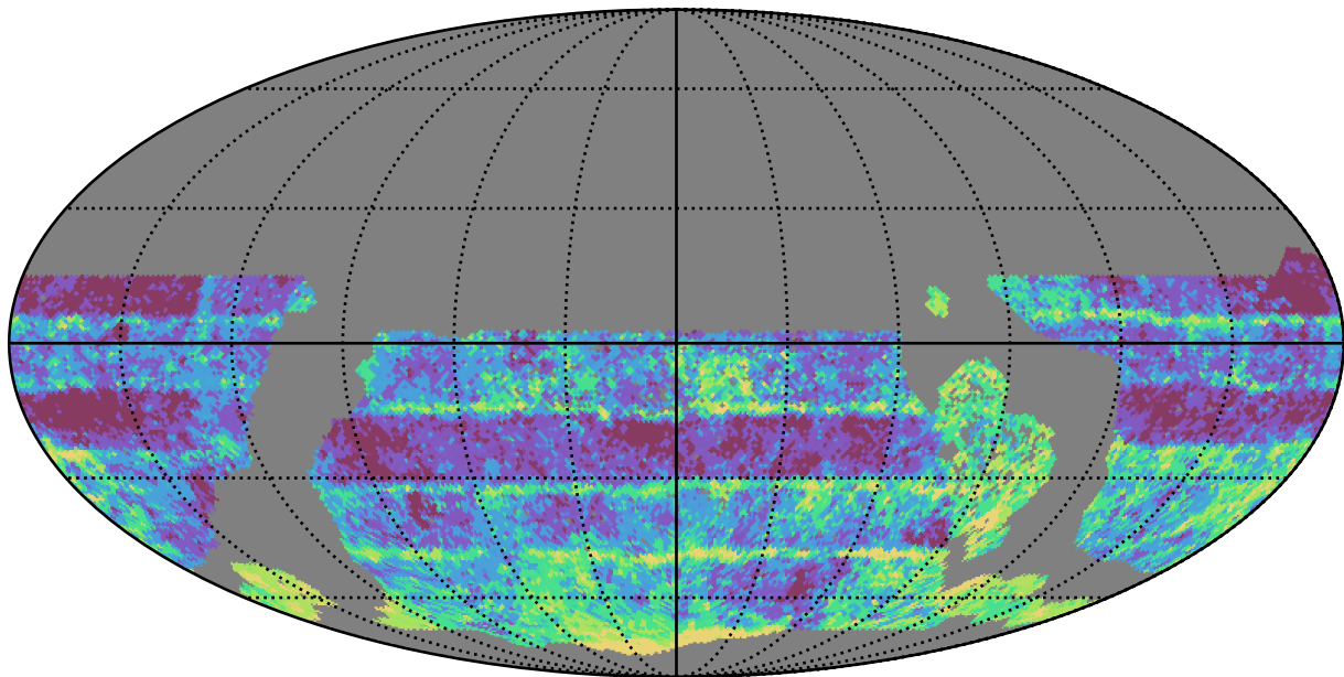
ddf_acor_sf15_lsf20_lsr50_v3.4_10yrs WFD r band: Median Inter-Night Gap
