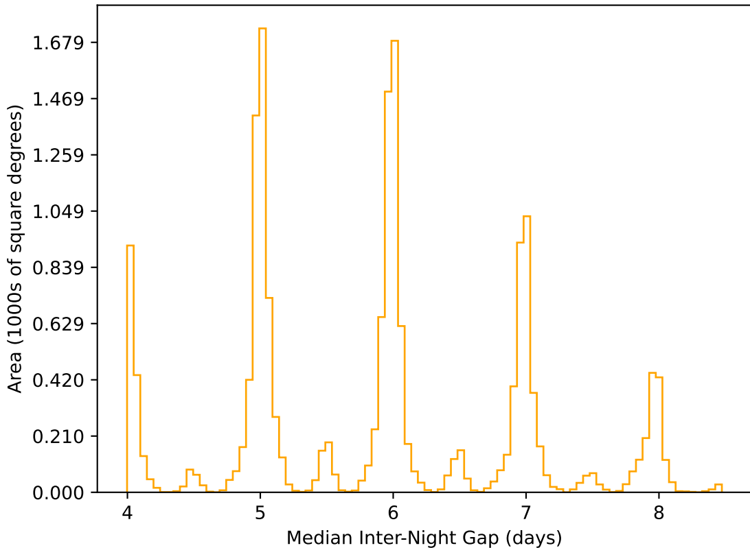
ddf_acor_sf15_lsf20_lsr50_v3.4_10yrs WFD r band: Median Inter-Night Gap
