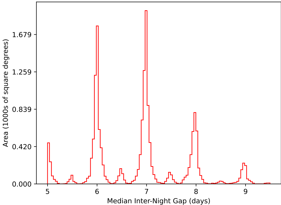
ddf_acor_sf15_lsf20_lsr50_v3.4_10yrs WFD i band: Median Inter-Night Gap
