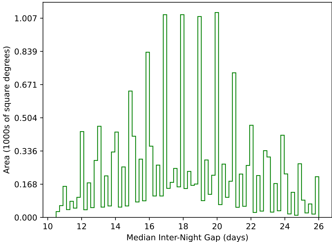
ddf_acor_sf15_lsf20_lsr50_v3.4_10yrs WFD g band: Median Inter-Night Gap
