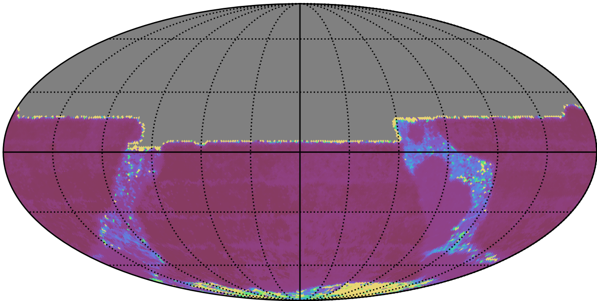
ddf_acor_sf15_lsf20_lsr50_v3.4_10yrs All sky y band: Median Inter-Night Gap
