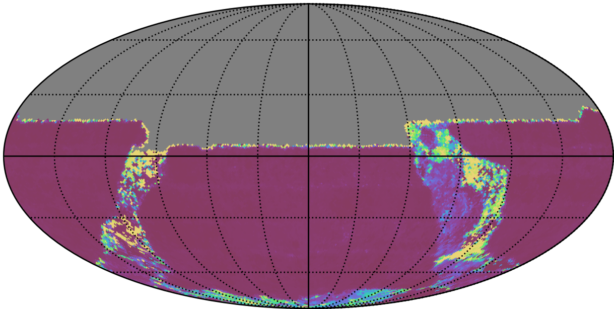
ddf_acor_sf15_lsf20_lsr50_v3.4_10yrs All sky u band: Median Inter-Night Gap
