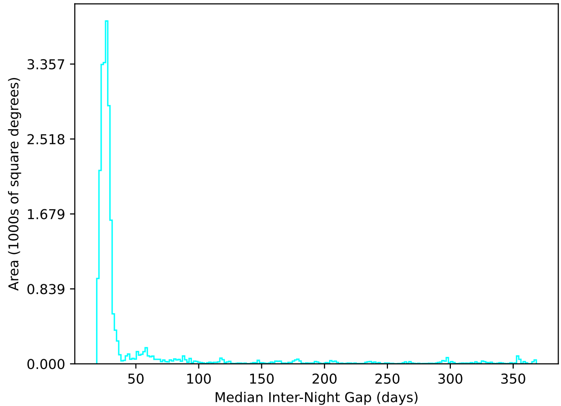
ddf_acor_sf15_lsf20_lsr50_v3.4_10yrs All sky u band: Median Inter-Night Gap
