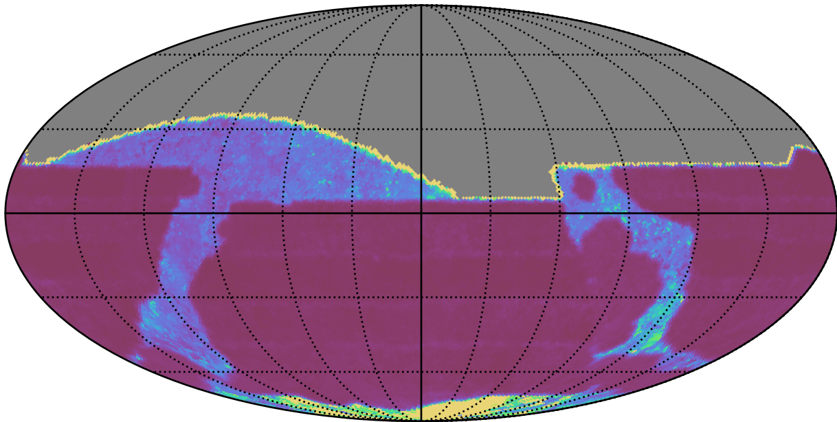
ddf_acor_sf15_lsf20_lsr50_v3.4_10yrs All sky r band: Median Inter-Night Gap
