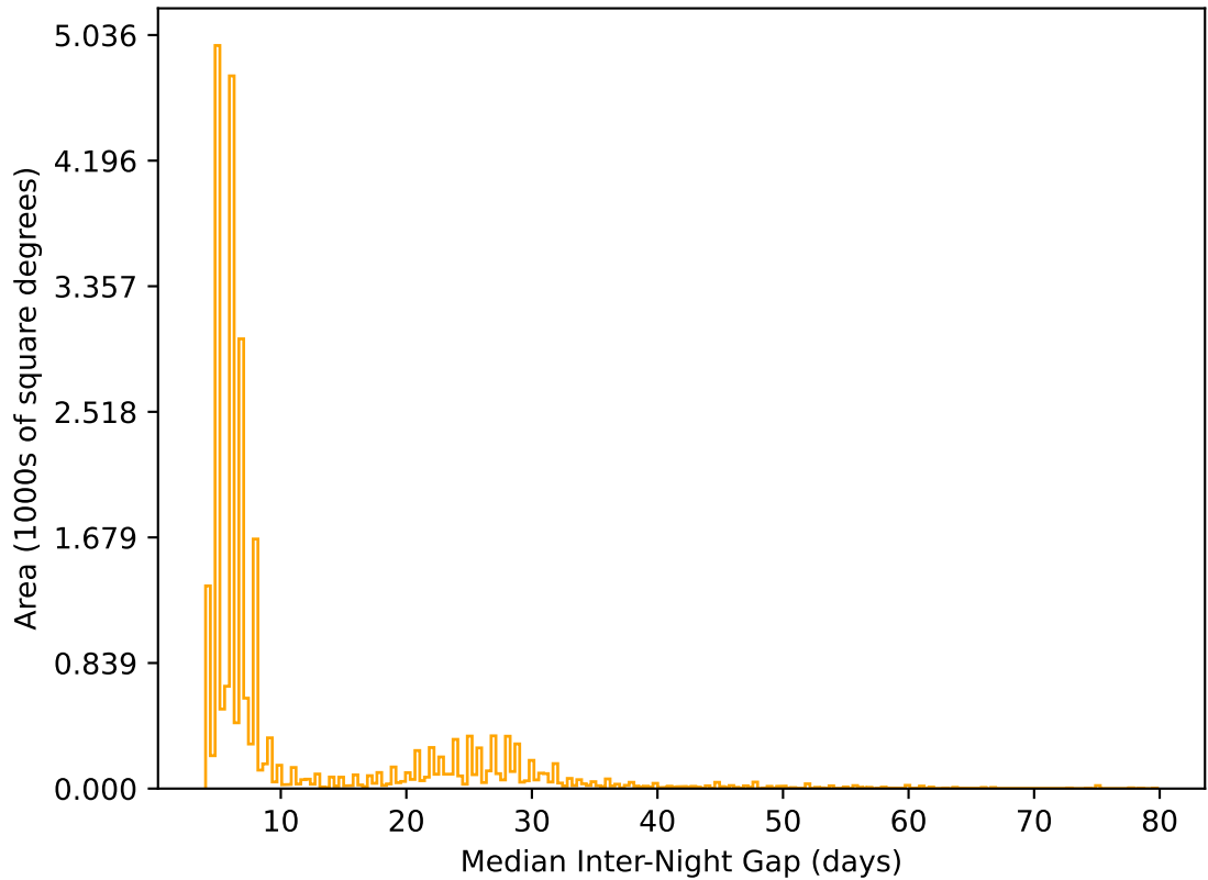
ddf_acor_sf15_lsf20_lsr50_v3.4_10yrs All sky r band: Median Inter-Night Gap
