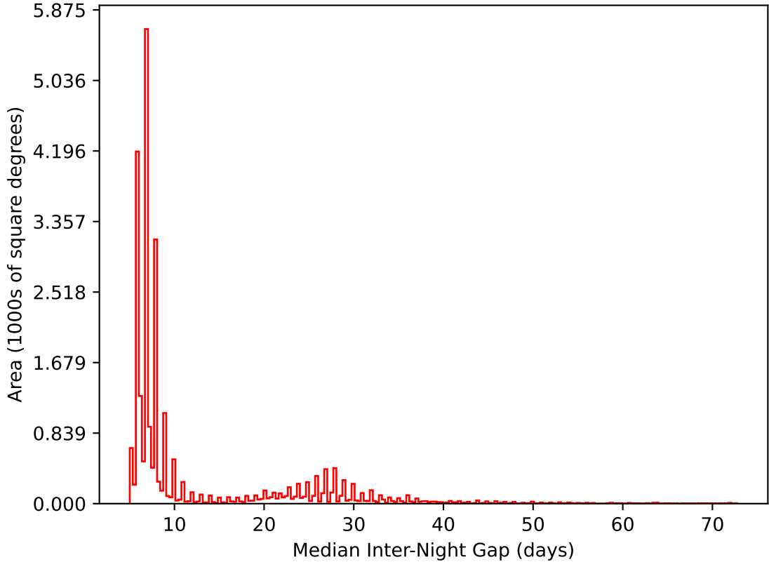
ddf_acor_sf15_lsf20_lsr50_v3.4_10yrs All sky i band: Median Inter-Night Gap
