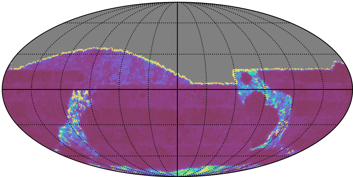
ddf_acor_sf15_lsf20_lsr50_v3.4_10yrs All sky g band: Median Inter-Night Gap
