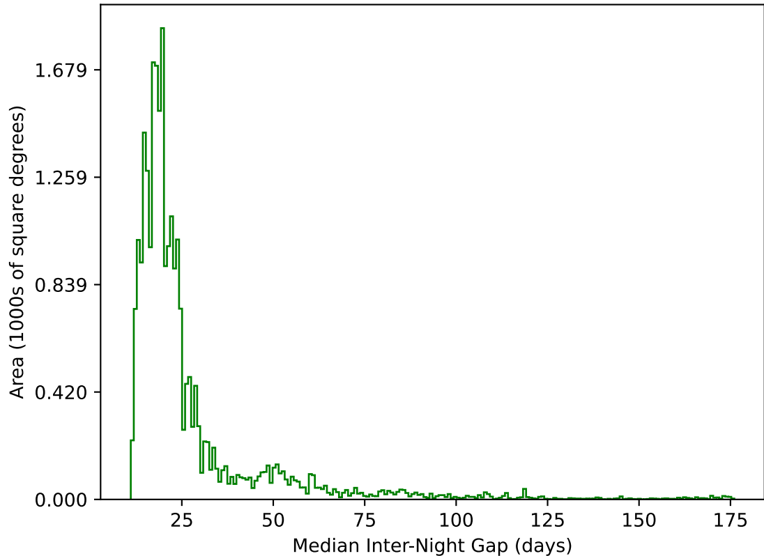
ddf_acor_sf15_lsf20_lsr50_v3.4_10yrs All sky g band: Median Inter-Night Gap
