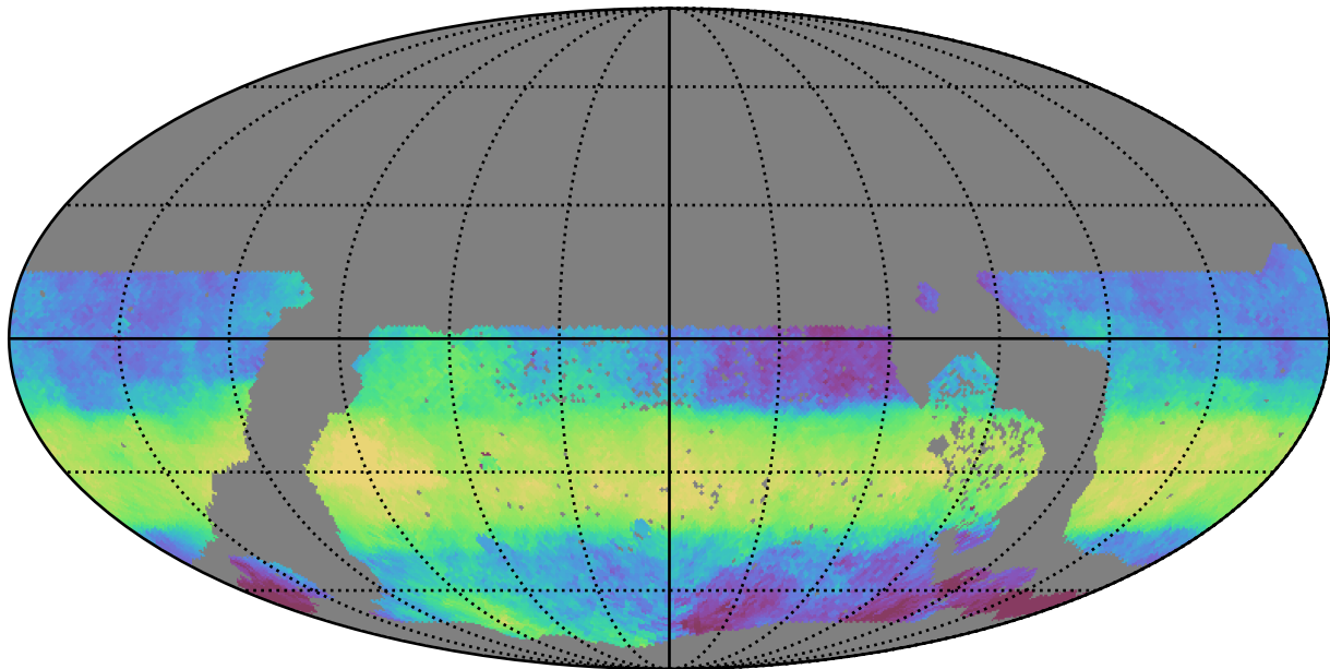
ddf_acor_sf15_lsf20_lsr50_v3.4_10yrs WFD z band: Median HA
