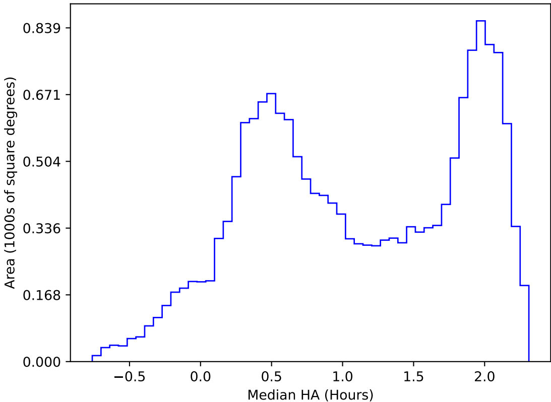
ddf_acor_sf15_lsf20_lsr50_v3.4_10yrs WFD z band: Median HA
