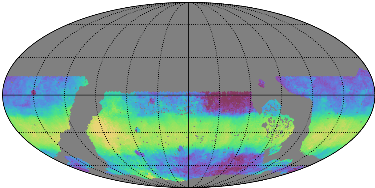
ddf_acor_sf15_lsf20_lsr50_v3.4_10yrs WFD y band: Median HA
