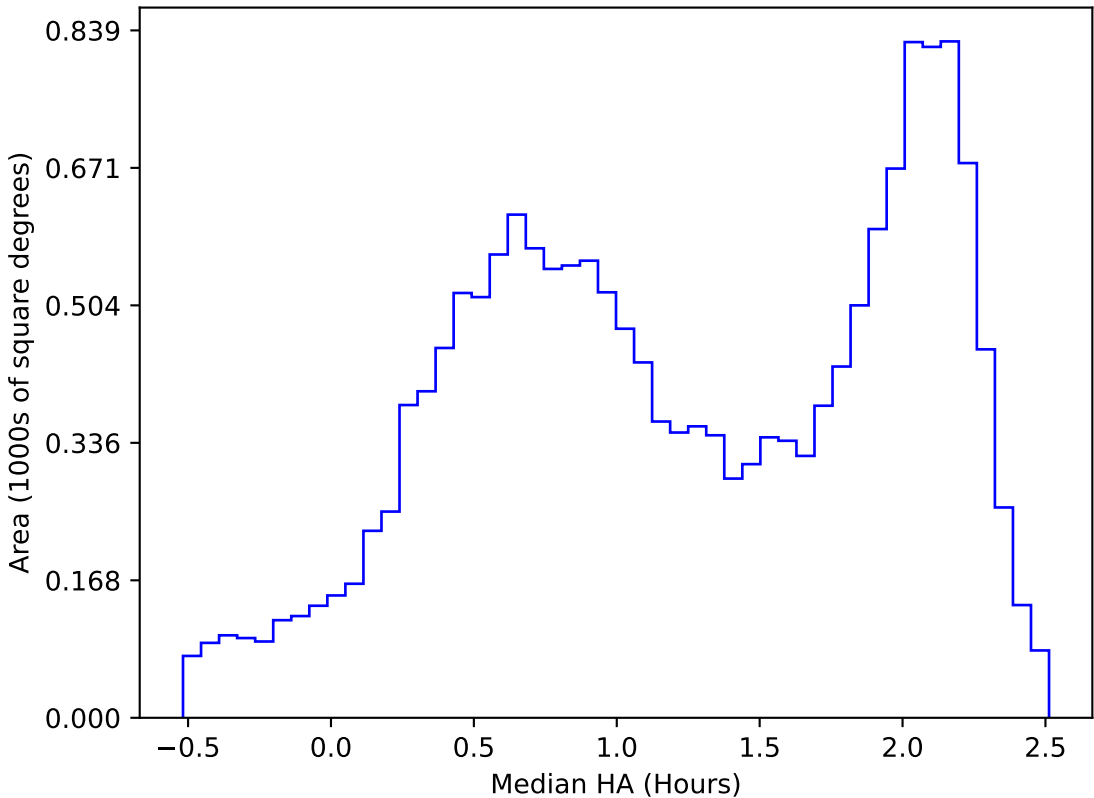
ddf_acor_sf15_lsf20_lsr50_v3.4_10yrs WFD y band: Median HA
