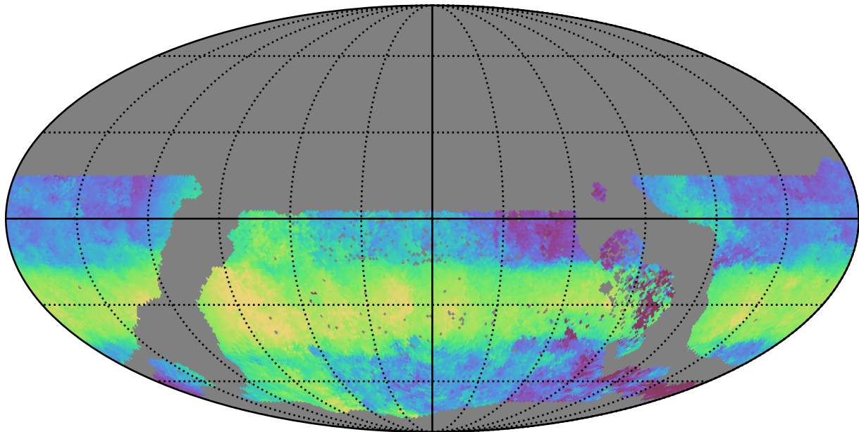
ddf_acor_sf15_lsf20_lsr50_v3.4_10yrs WFD u band: Median HA
