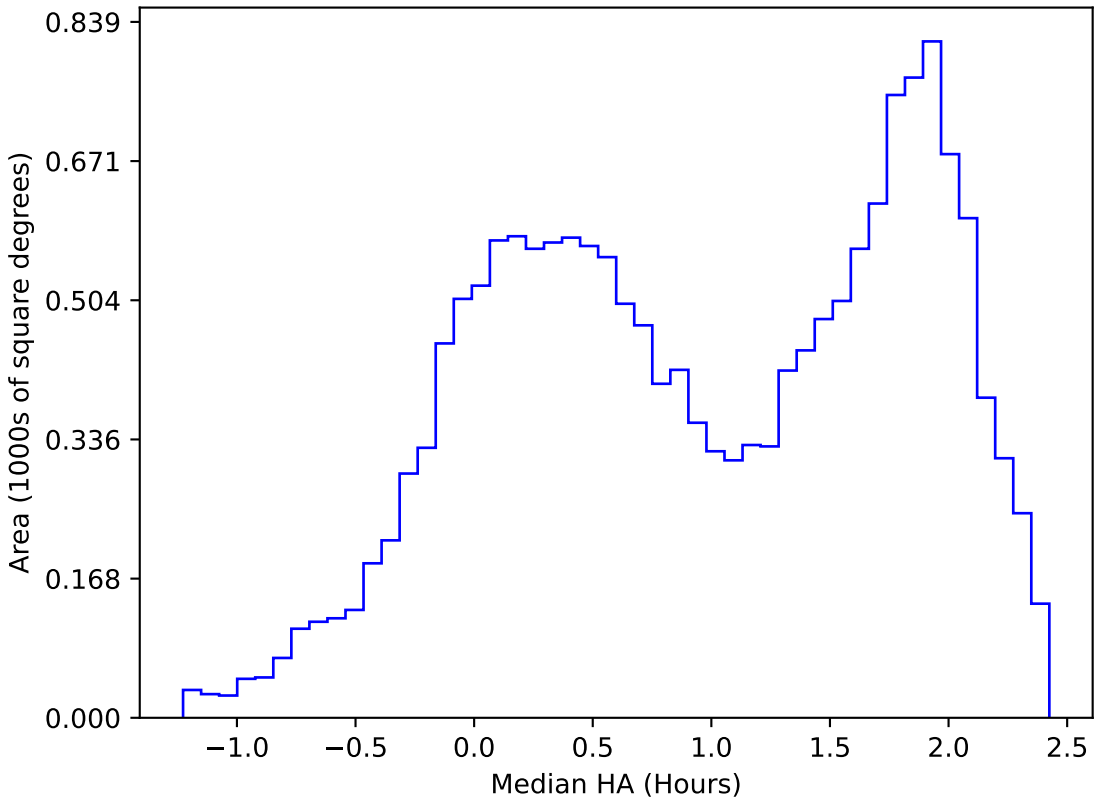
ddf_acor_sf15_lsf20_lsr50_v3.4_10yrs WFD u band: Median HA
