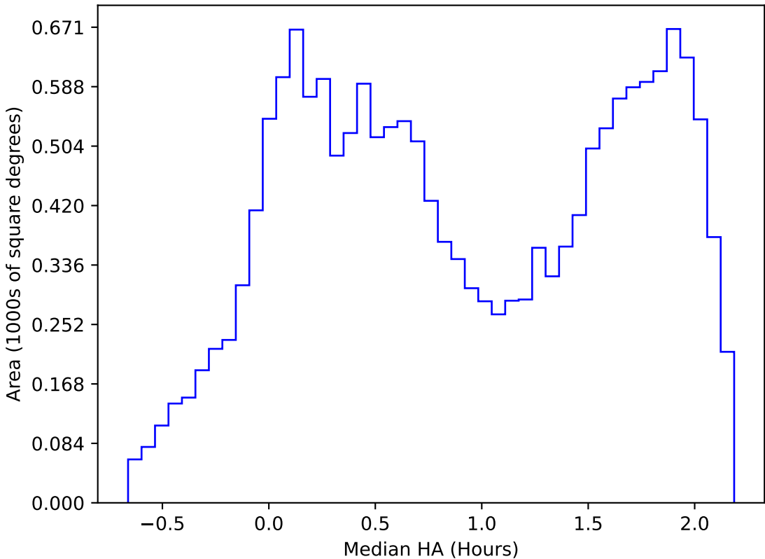
ddf_acor_sf15_lsf20_lsr50_v3.4_10yrs WFD r band: Median HA
